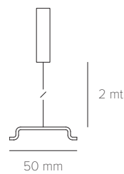
19030 Support with 200 cm wire
